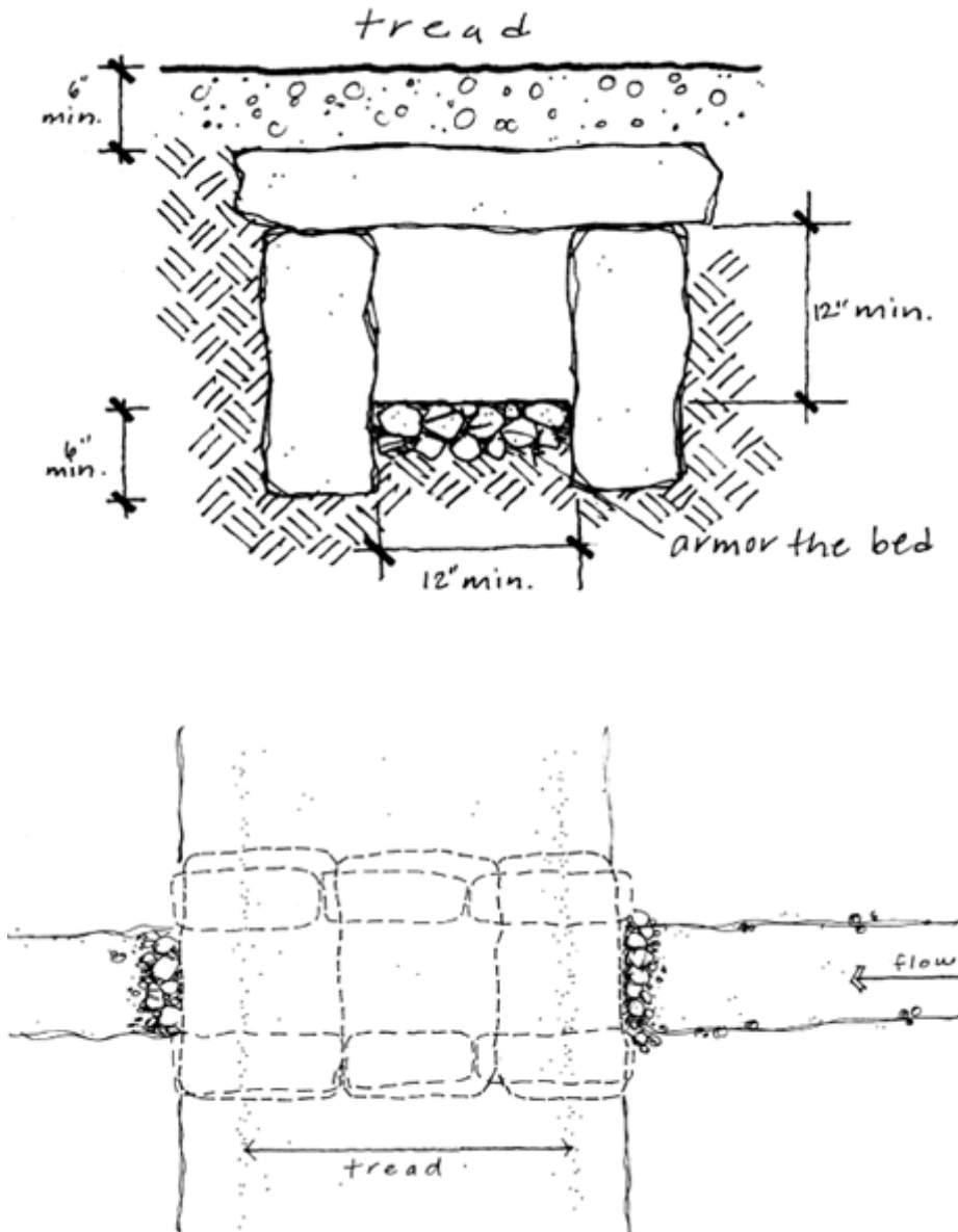
FIGURE 8-3.8 ROCK CULVERT
