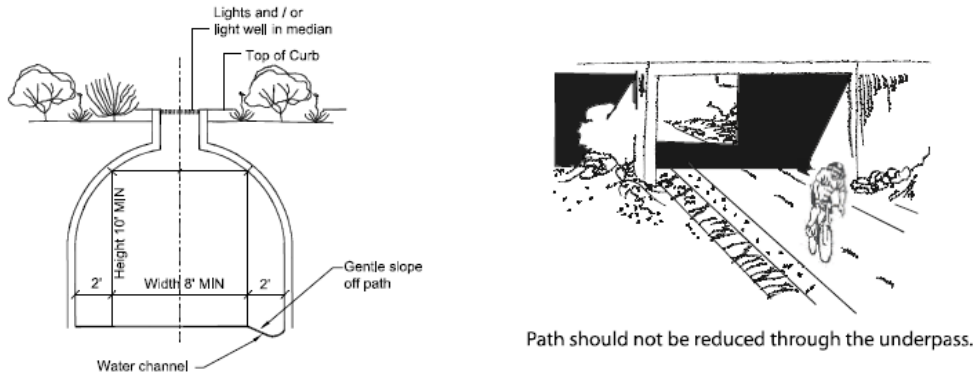
FIGURE 5-7.11 SHARED USE OR MULTIUSE PATH – TUNNELS
