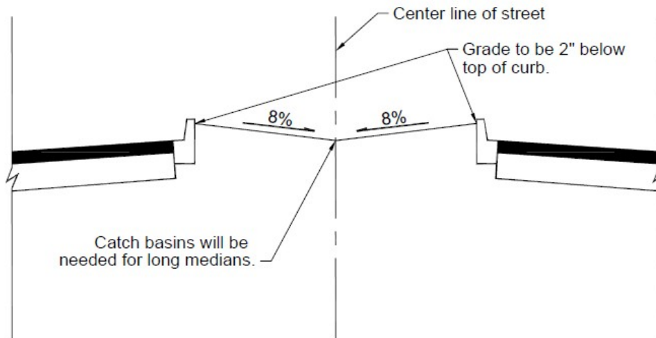
FIGURE 5-3.23 MEDIAN GRADING300
