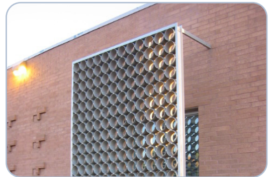
Sun screens can be incorporated into building architecture to reduce heat absorption.
